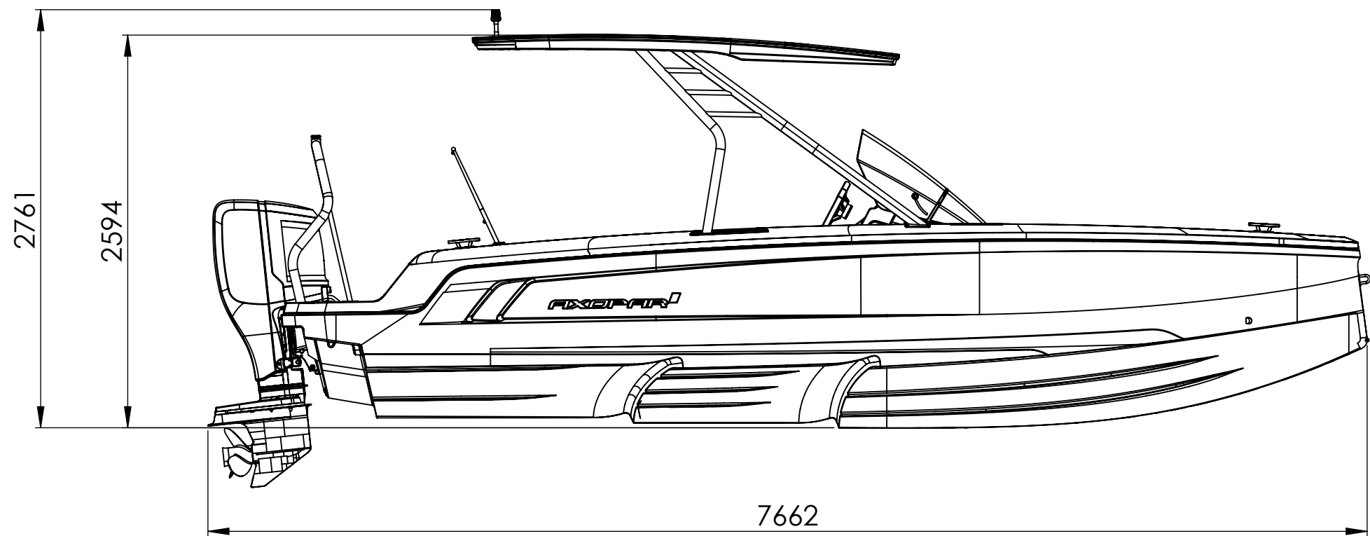
SIDE VIEW
