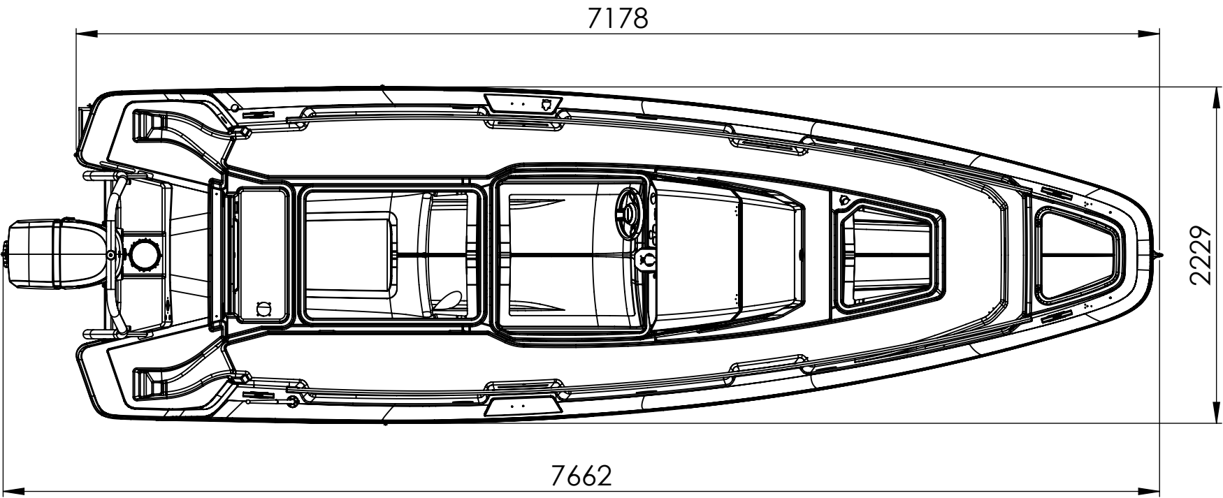
TOP VIEW
